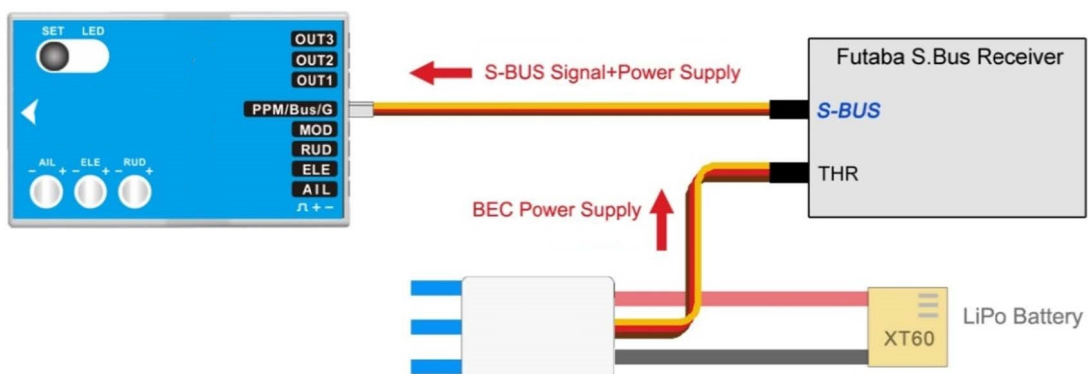
Futaba S-BUS / S-BUS 2 Connection
